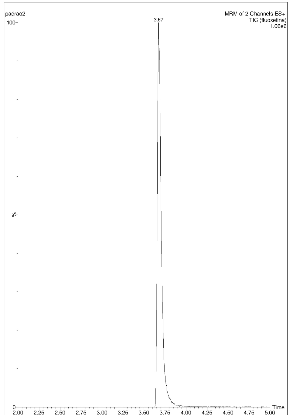
FIGURE S1 | Chromatogram of the fluoxetine hydrochloride standard at the concentration of 1 mg L -1 .
