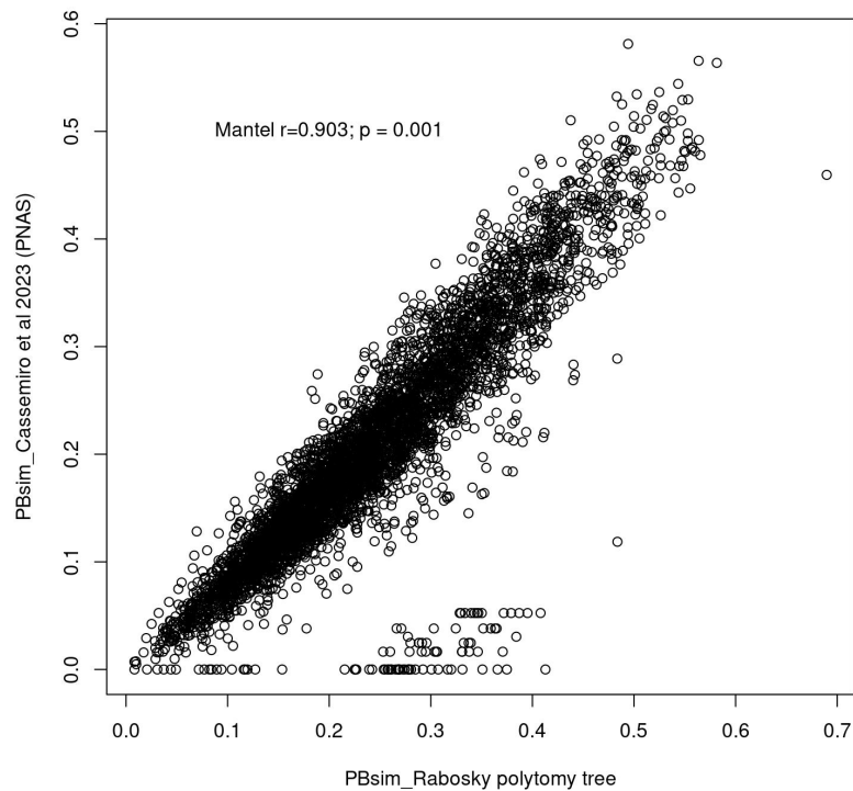
FIGURE S1 | Mantel correlation between PhyloBsim calculated with AmazonFISH taxonomic data and two distinct phylogenetic informations: Rabosky et al. (2018) (which includes genetic + polytomies based on taxonomy) and Cassemiro et al. (2023) (which include only genetic data).
