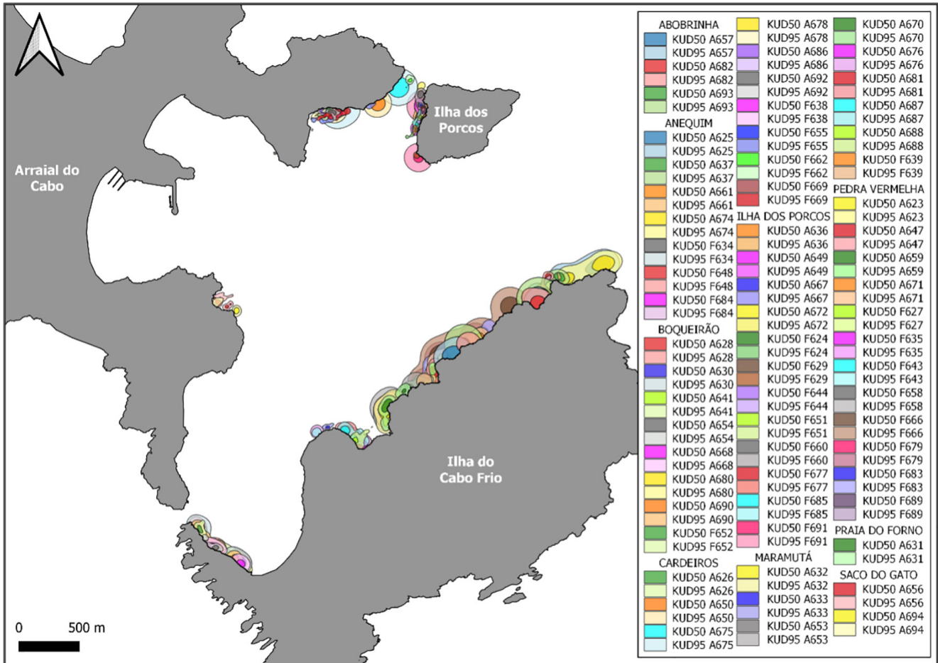
FIGURE S6 | Home range of all tagged Sparisoma axillare and S. frondosum calculated with the Kernel Utilization Distribution (KUD 95 and KUD 50) in Arraial do Cabo. The combination of letters and numbers in the right column in the legend refer to individual IDs of each fish.
