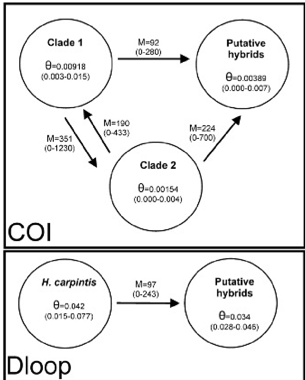
FIGURE S3 | Gene flow among populations of Herichthys carpintis and putative hybrids according to the most probable model recovered in Bayes Factor analysis. Theta values and 95% HPD intervals are shown within each genetic cluster. The values on the arrows show the number of migrants from one population to another with the 95% HPD in parentheses.
