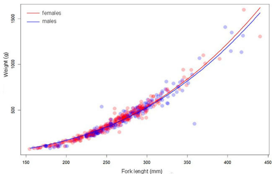
FIGURE S1 | Length x weight relationship of males and females gray triggerfish, Balistes capriscus , captured in southeast Brazil.
