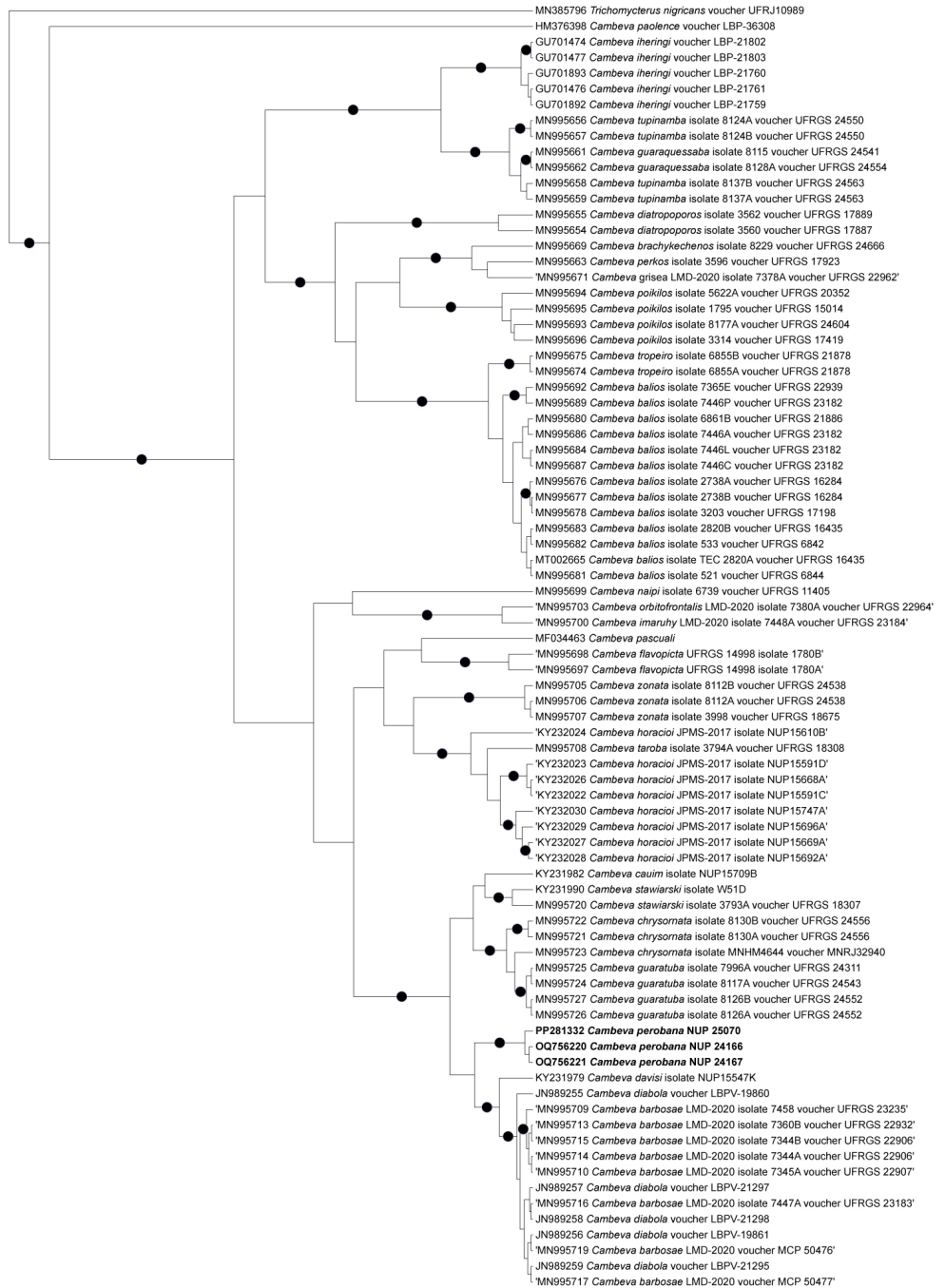
FIGURE S1 | Bayesian COI gene tree of Cambeva without collapsed clades. Circles represent posterior probability = or > 0.95.
