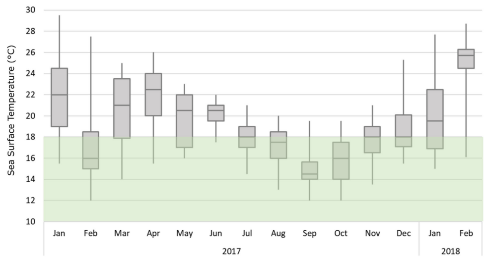
FIGURE S1 | Sea surface temperature (SST) recorded with a data logger (HOBO Tidbit UTBI-001) fixed at 1 m deep in the rocky shores of Praia Grande, Arraial do Cabo, Rio de Janeiro (PELD-RECA). Area in green ( \leq 18 °C) are considered under the influence of upwellings of SACW (South Atlantic Central Water).
