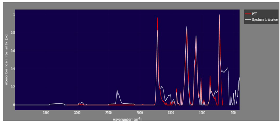
FIGURE S9 | Fiber absorbance spectrum using micro-FTIR technique, r = 0.94 (Open Specy reference database).
