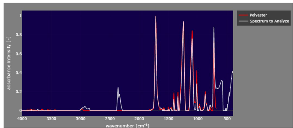
FIGURE S7 | Fiber absorbance spectrum using micro-FTIR technique, r = 0.85 (Open Specy reference database).
