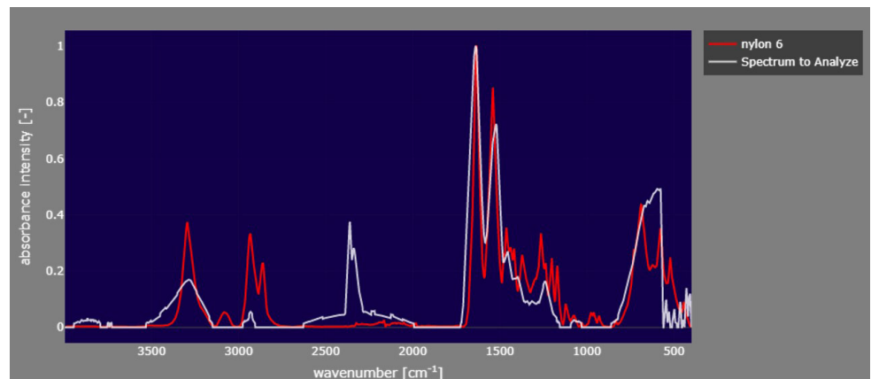
FIGURE S6 | Fiber absorbance spectrum using micro-FTIR technique, r = 0.79 (Open Specy reference database).
