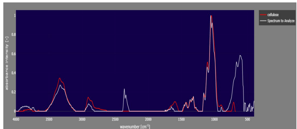
FIGURE S11 | Fiber absorbance spectrum using micro-FTIR technique, r = 0.94 (Open Specy reference database).
