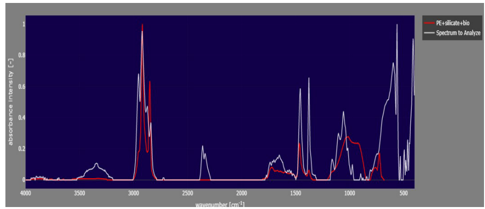
FIGURE S10 | Fiber absorbance spectrum using micro-FTIR technique, r = 0.74 (Open Specy reference database).
