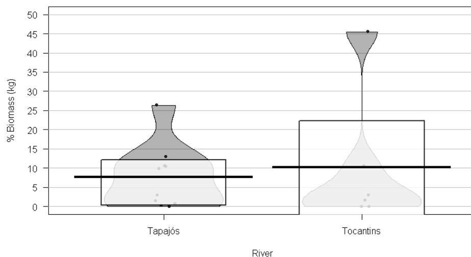
FIGURE S1 | Comparison of mean relative abundance (% of biomass in kg) of Plagioscion squamosissimus sampled in the Tapajós (n = 9) and Tocantins rivers (n = 5). Mean (dark vertical line), data distribution (bean gray area), data (points), confidence interval (rectangle). Points indicate the sampling sites (fishing communities), considered as replicates in this analysis. The statistical t-test was conducted with log-transformed data, but the graph shows the original data.
