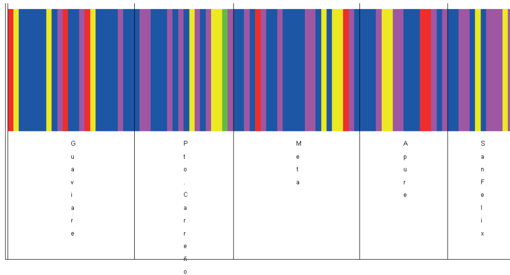
FIGURE S14 | Barplots using BAPS representing assignment of individuals to populations of Piaractus orinoquensis .
