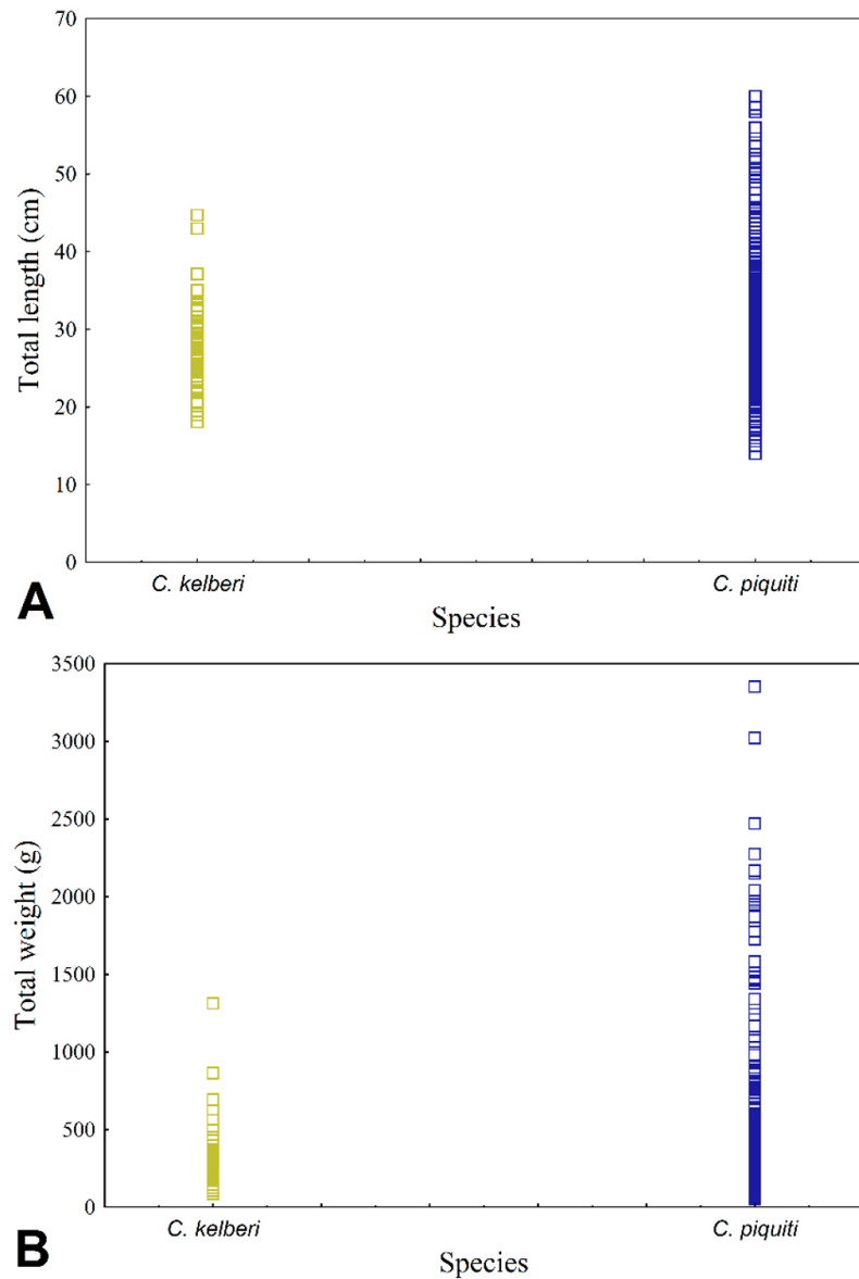
FIGURE S3 | Variations in total length (A) and total weight (B) of Cichla kelberi and C. piquiti . Each dot is a fish.
