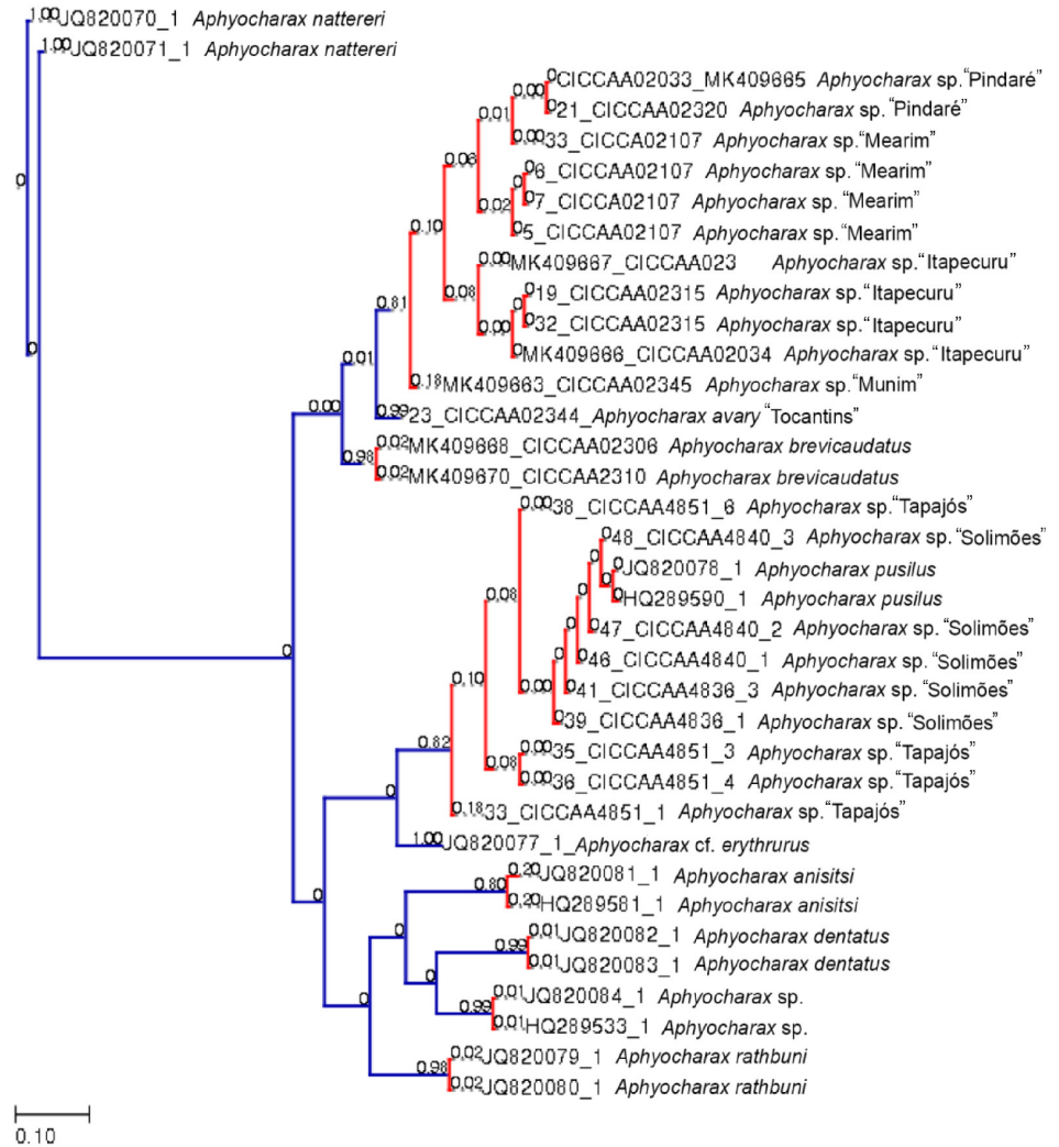
FIGURE S2 | bPTP test analysis. We found the same result to the ingroup, when compared to the result presented in Fig. 3.
