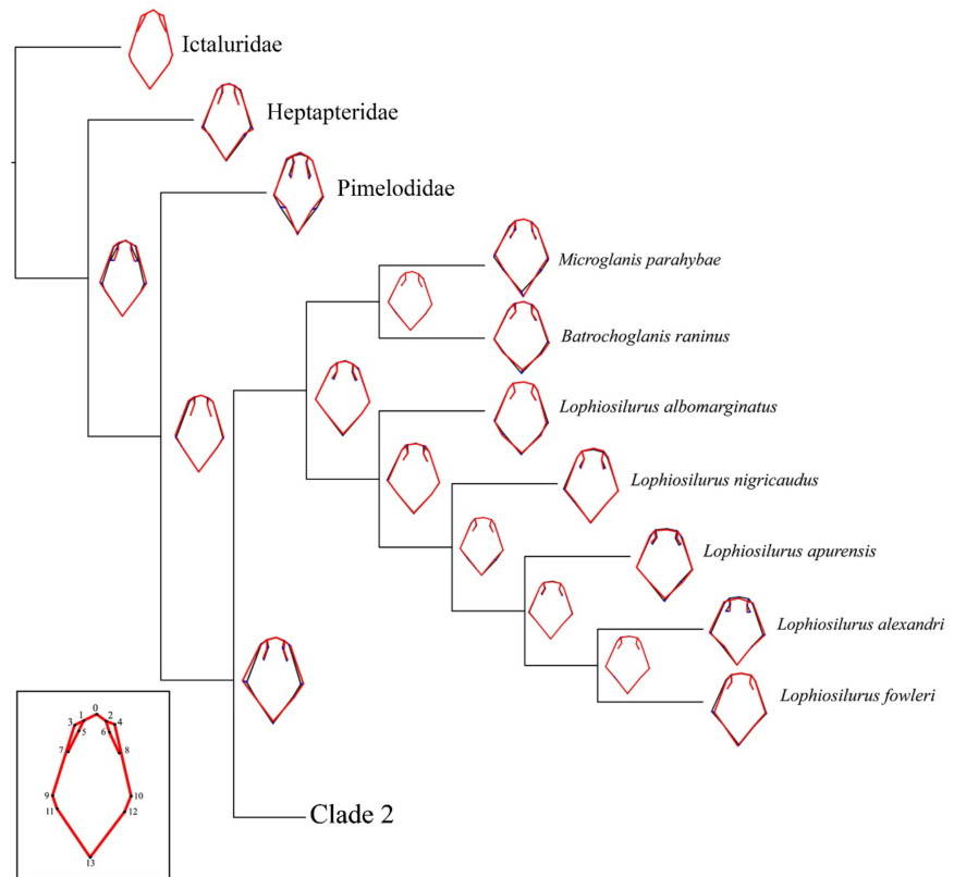
FIGURE S3 | Landmark mapping on Pseudopimelodidae phylogeny (Outgroups plus Clade 1: Batrochoglaninae). Inferred phylogeny and landmarks mapping on the head of Batrochoglaninae (Clade 1: Microglanis , Batrochoglanis , and Lophiosilurus ). The ancestral shape is indicated in grey dotted lines; reconstructed shape in red lines, blue lines showing the change in position of each landmark to the corresponding node in the ancestor. The ancestral configurations are also indicated on the nodes. In the box are enumerated landmarks on the enlarged image of Ictalurus punctatus .
