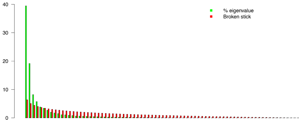
FIGURE S3 | Significant eigenvalues derived from the Fourier matrix determined by the “Broken-Stick” method for the populations of Cichla temensis .
