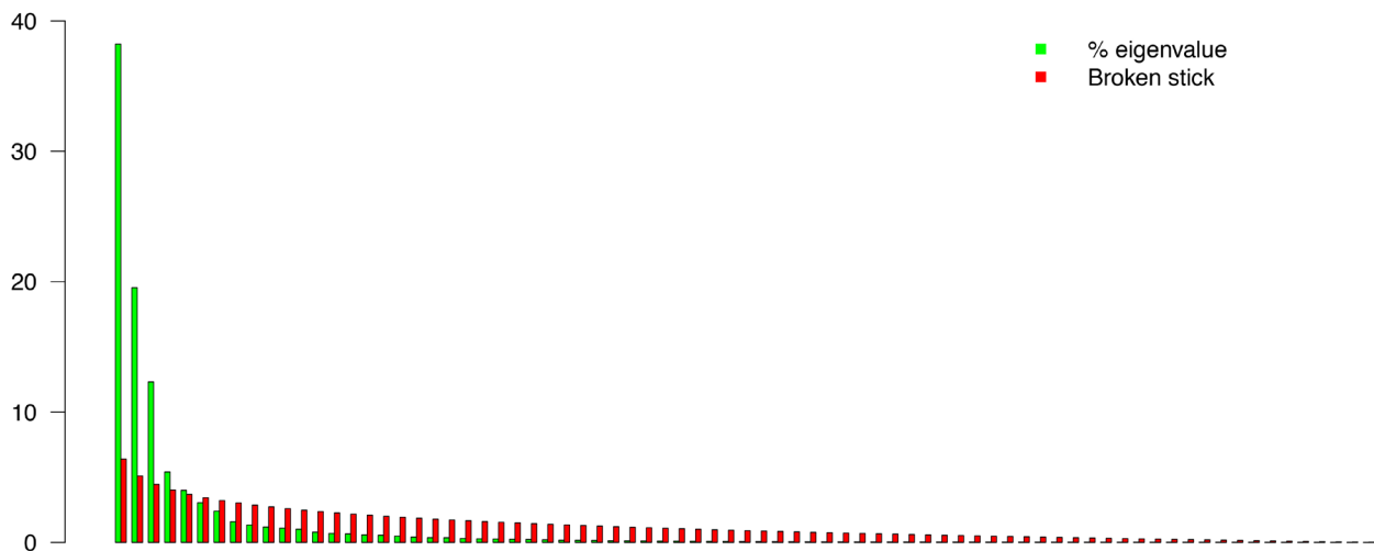
FIGURE S2 | Significant eigenvalues derived from the Fourier matrix determined by the “Broken-Stick” method for Cichla species.
