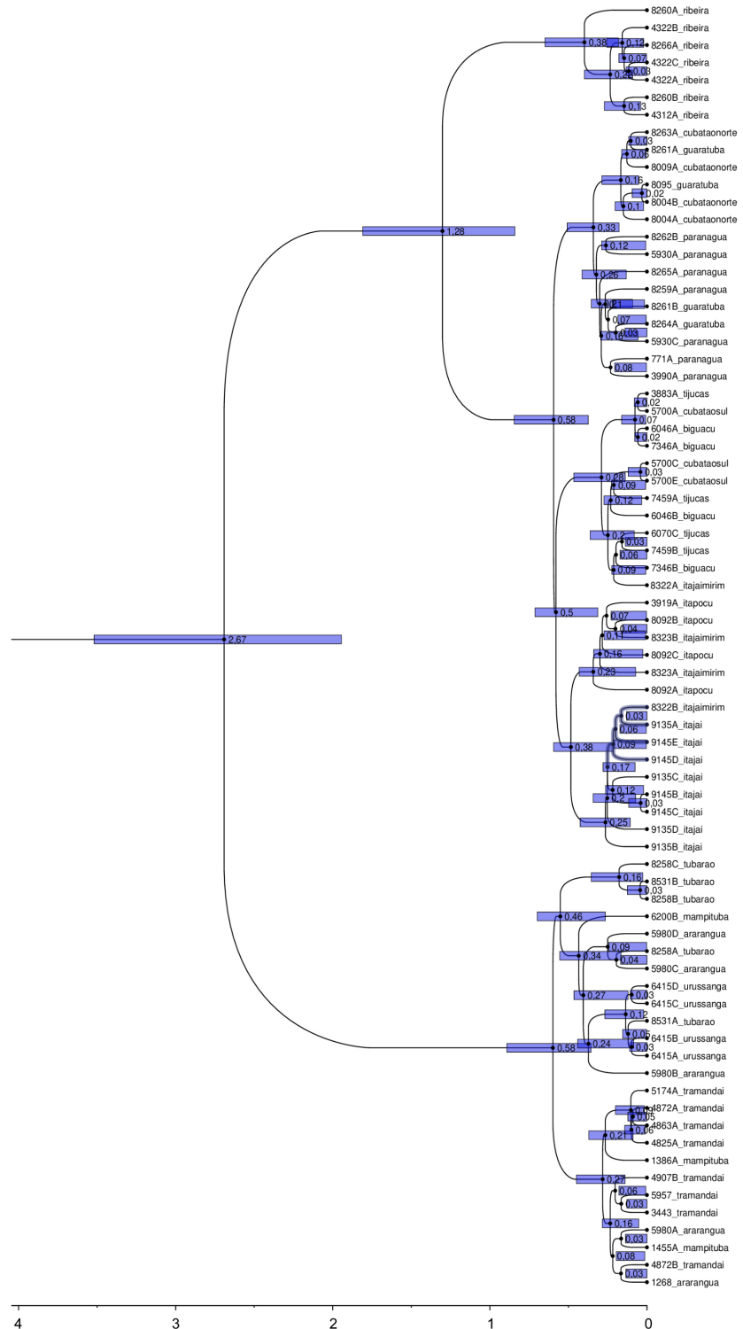
FIGURE S3 | Phylogeny of Hisonotus leucofrenatus for nuclear rpS7 ribosomal protein gene intron samples with all terminals included.
