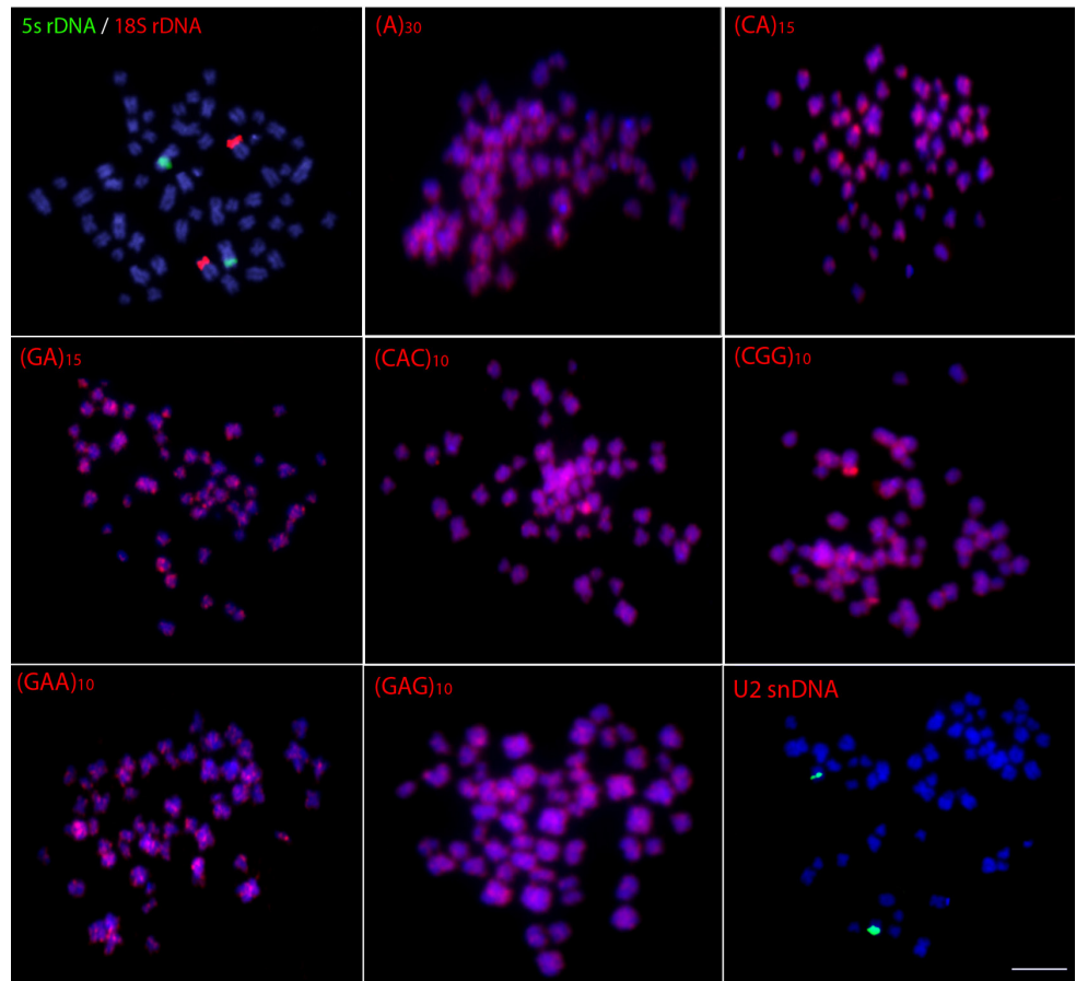
SUPPLEMENTARY MATERIAL FIGURE S3 | Metaphase plates of Arapaima gigas from São Félix do Araguaia (SFA) population (Araguaia-Tocantins River basin) hybridized with repetitive DNA sequences, including mono-, di- and trinucleotide microsatellites and the multigene families U2 snDNA. Bar=5 \mu m.
